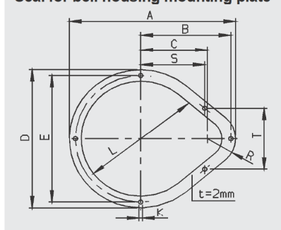
Seal for bell housing mounting plate
