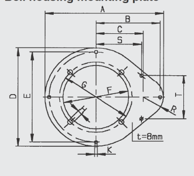
Bell housing mounting plate
