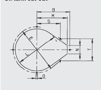
Oil tank cut-out
